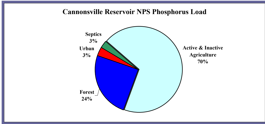
Figure 2. "NPS load by land use," Data for chart provided by Porter, 2001.
