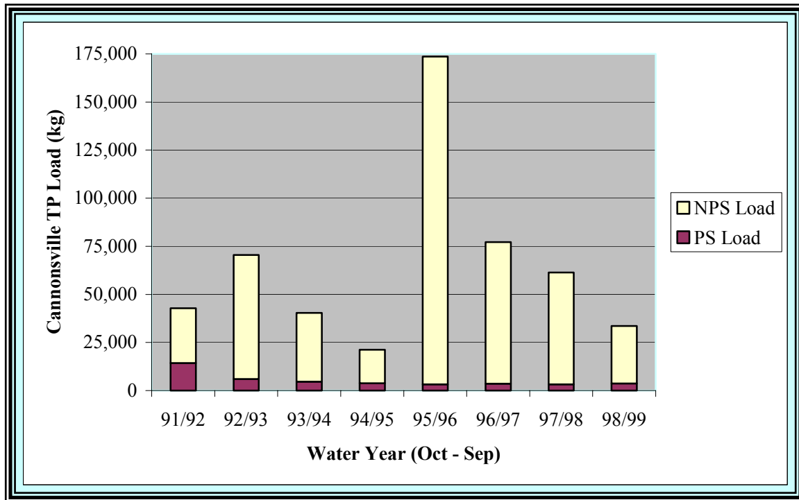
Figure 1. Point source (PS) and Non-Point Source (NPS) Loads in the Cannonsville Reservoir
